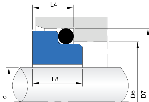
O-ring mounted seats,with standard dimensions. Material: V1, Q1, Q2, U2 A.B
